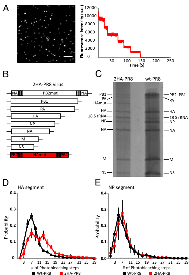
Fig. 3. PR8 virus particle packages one copy of the HA segment. (A) Photobleaching analysis of the HA viral RNA in PR8 viruses hybridized with 15 Cy5-labeled probes. Right , An average of 30,000 TIRF movie frames of a short movie taken at an imaging area which was consistently excited for 5 min. The graph represents a typical plot of total fluorescence intensity versus time for a Cy5 spot exhibiting a seven-step photobleaching behavior. This plot corresponds to the circled spots in the averaged TIRF image ( Left ). (B) Genome structure of the 2HA-PR8 virus. Seven A/Puerto Rico/8/34 ambisense plasmids (pDZ-PB1, pDZ-PA, pDZ-HA, pDZ-NP, pDZ-NA, pDZ-M, pDZ-NS) and two chimeric constructs, pDZ-NA-PB2mut-NA and pDZ-PB2-HAmut-PB2 ( Material and Methods ) were used to generate the 2HA-PR8 virus by reverse genetics. (C) Analysis of viral RNA packaging in 2HA-PR8 virus. Purified viral RNAs from the 2HA-PR8 virus and PR8 virus were resolved using a 2.8% acrylamide gel, followed by silver staining. The identities of the bands were labeled based on their sizes and previous findings. (D) Histogram of the photobleaching steps analyzed for the FISH probes hybridized HA segment in PR8 and 2HA-PR8 viruses. Error bars denote SDs ( n \geq 5 ). (E) Histogram of the photobleaching steps analyzed for the FISH probes hybridized NP viral RNA in PR8 virus and 2HA-PR8 virus. The black squares and solid black lines represent the PR8 virus, and the red squares and solid red lines represent the 2HA-PR8 virus. Error bars denote SDs ( n \geq 3 ).
